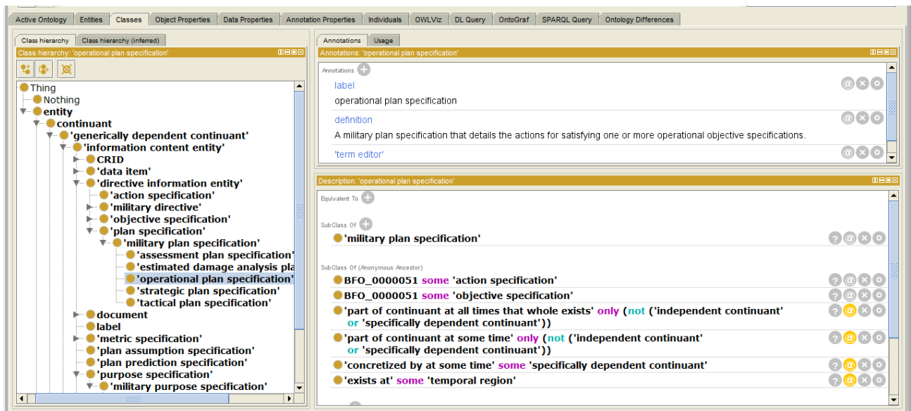
Figure 1: Draft of the Plan Ontology at http://ncor.buffalo.edu/plan-ontology
